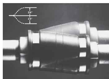
3. Parallel misalignment.
